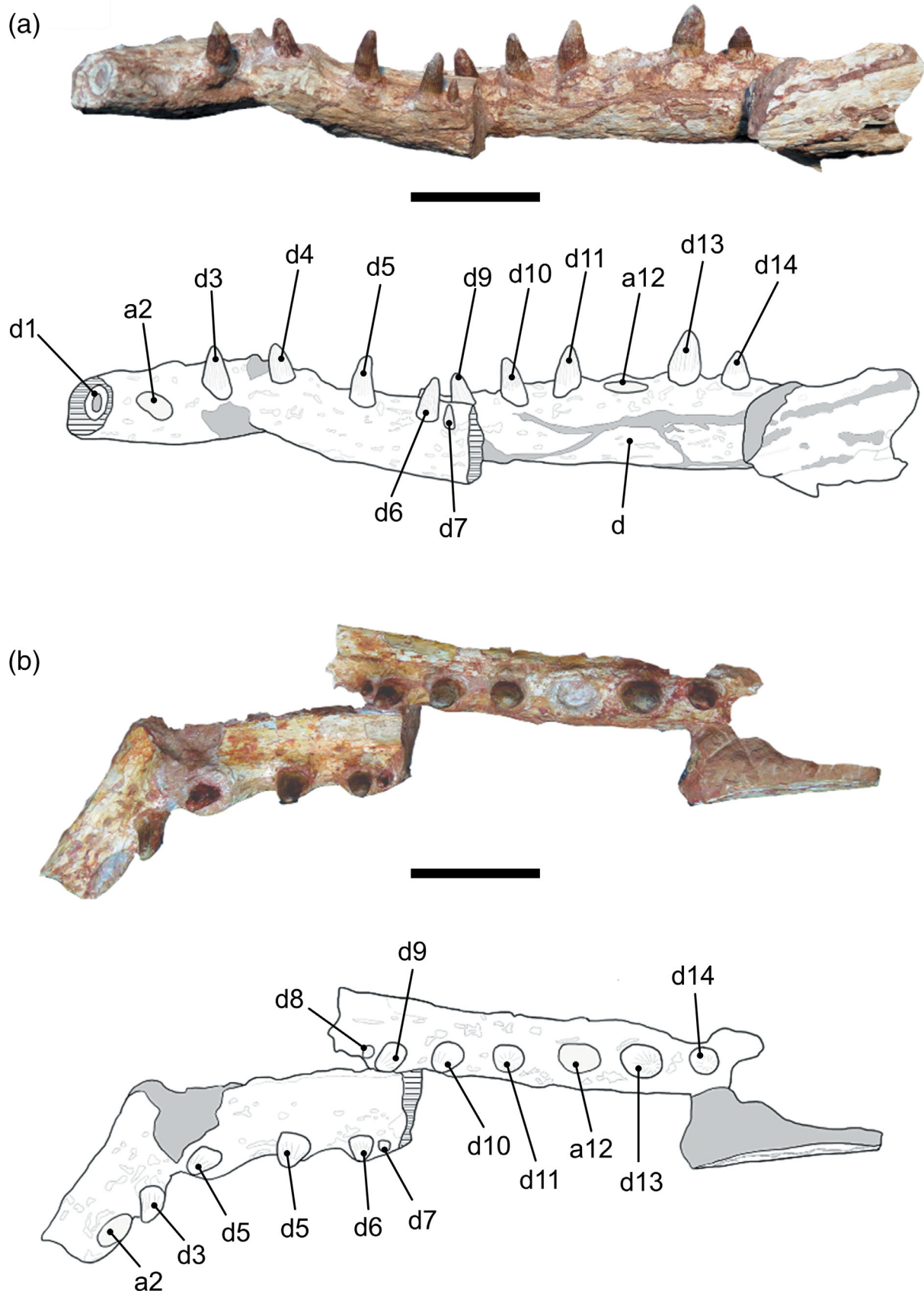
FIGURE 3 Left hemimandible of Epoidesuchus tavaresae gen. et sp. nov. MPMA 68-0001/11, holotype; interpretative drawings at right. (a) Left lateral view and (b) ocular view of hemimandible. a2–12, alveoli; d, dentary; d1–14; dentary teeth. Scale bars equal to 5 cm.
