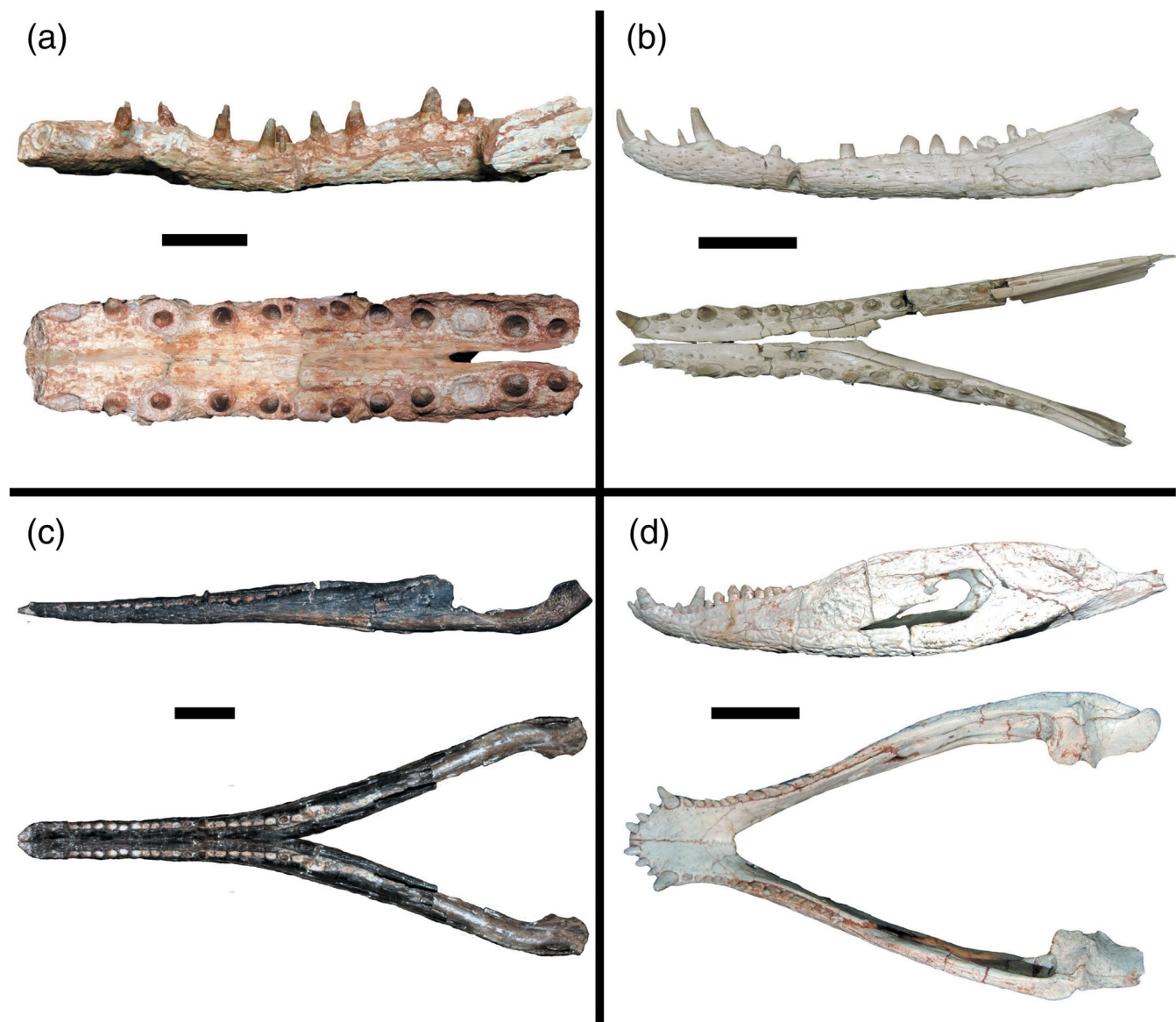
FIGURE 8 Lateral and dorsal views of the mandible of peirosaurids. (a) Epoidesuchus tavaresae MPMA 68-0001/11 (dorsal view reconstructed); (b) Pepesuchus deiseae MCT 1788-R; (c) Stoloekrosuchus lapparenti MNN GDF600 (dorsal view reconstructed); and (d) Montealtosuchus arrudacamposi MPMA-16-0007/04. Scale bars equal to 5 cm.
